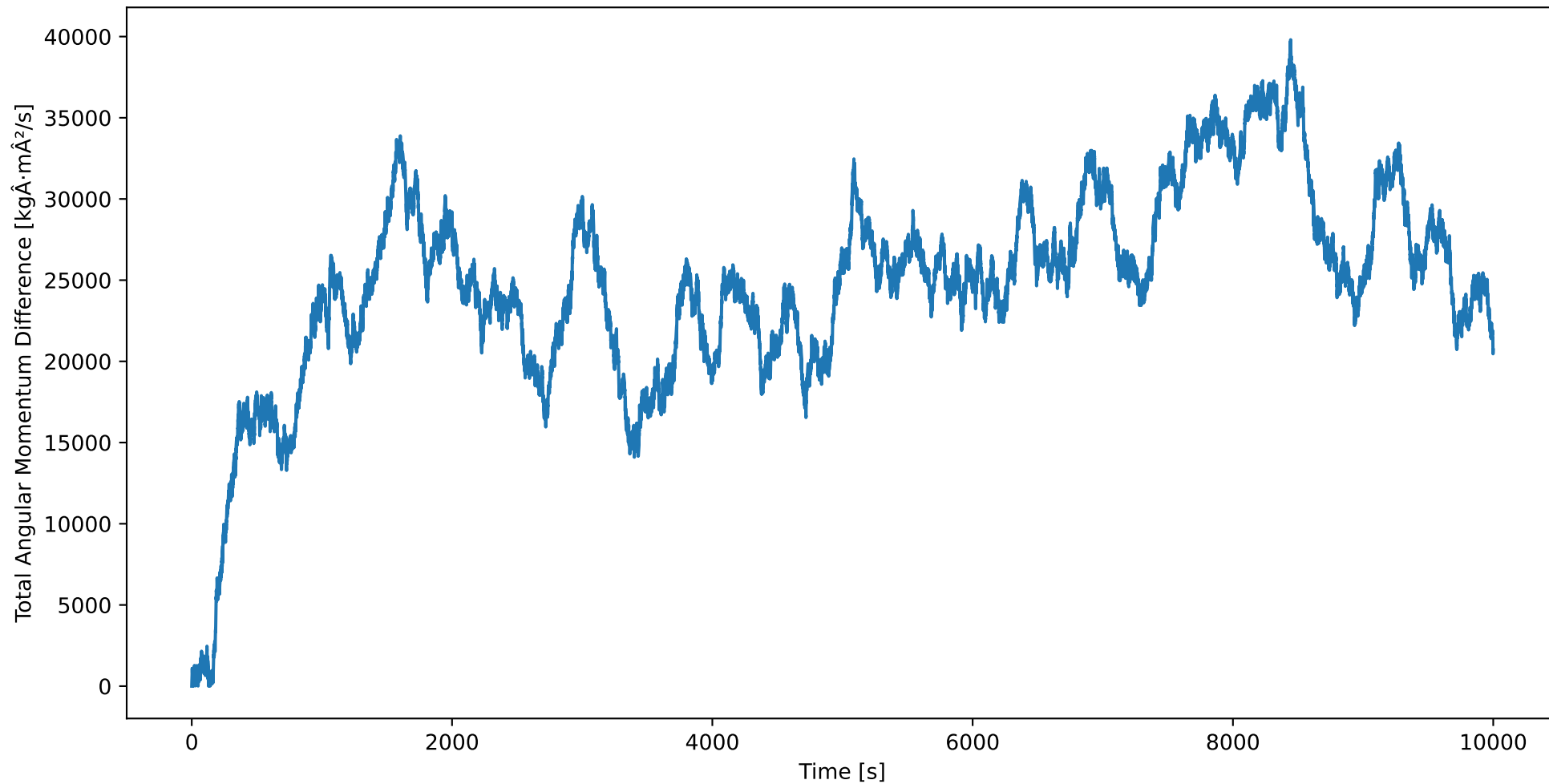
Total Angular Momentum Drift over time
